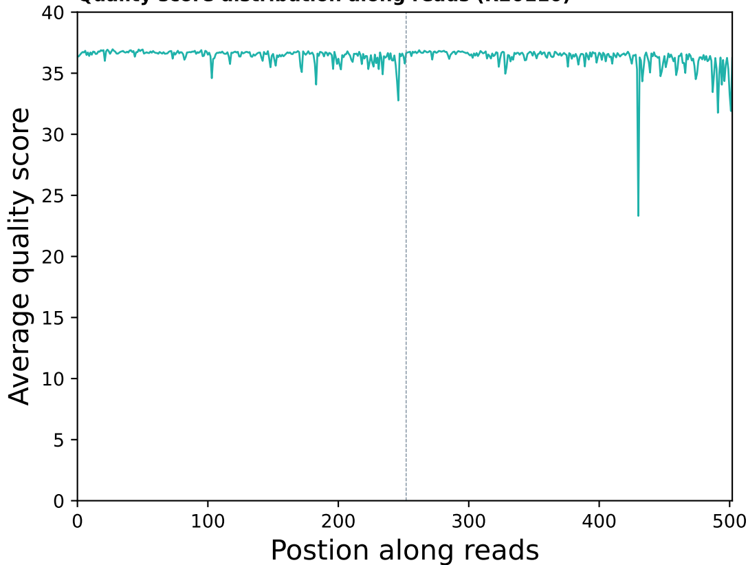
Quality score distribution along reads (R20110)
